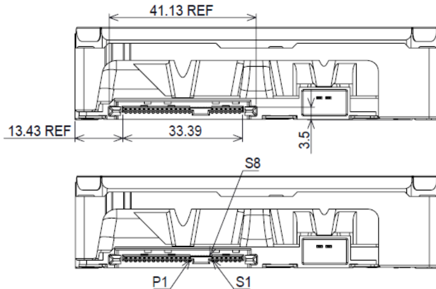
Figure 9 Connector locations
